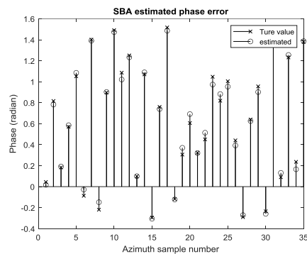
(شکل-۹): Added phase error to each azimuth and its estimation resulted by SBA method for 63% samples and SNR = 15dB.
