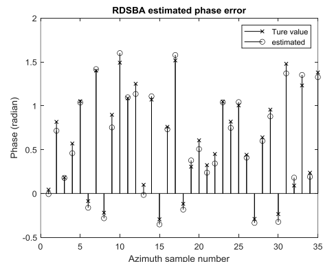
(شکل-۱۰): Added phase error to each azimuth and its estimation resulted by RDSBA method for 63% samples and SNR = 15dB.
