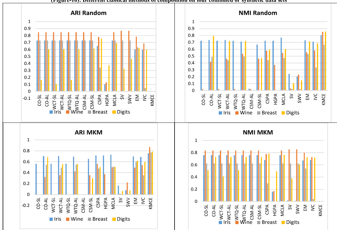
(Figure-10): Different classical methods of composition on four combined or synthetic data sets
