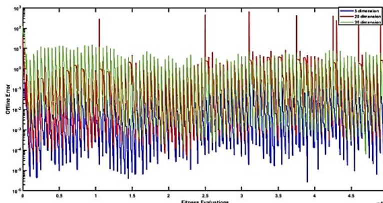
Figure (12): Offline error of the proposed method for dimensions of sizes 5, 20 and 30
