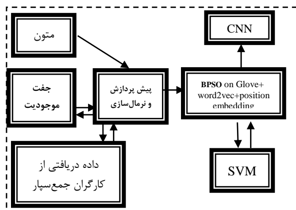
(Figure-1): Proposed model for classifying entities
