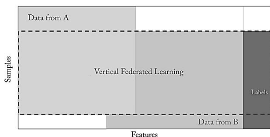
Illustration of Vertical Federated Learning, (Figure -4): a.k.a feature-partitioned federated learning where the overlapping data samples that have non-overlapping or partially overlapping features held by multiple participants are taken to jointly train a model.
