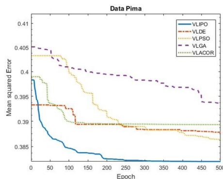
(Figure-24): Convergence of MSE value for Pima data set for simple ANFIS classifier
