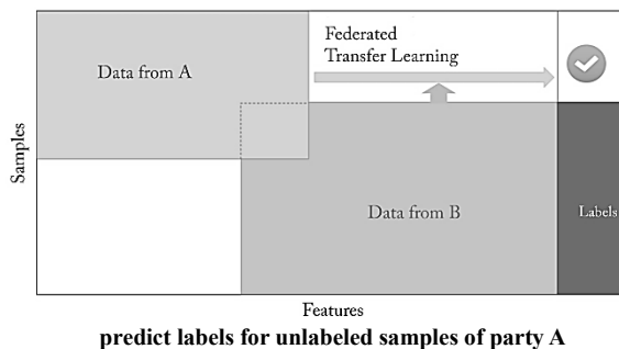
(Figure -6): Federated transfer learning (FTL). A predictive model learned from feature representations of aligned samples belonging to party A and party B is utilized to
