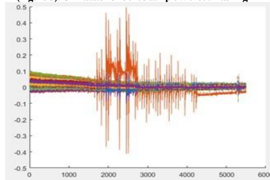
(Figure-5): CPA attack on 30208 sample without masking
