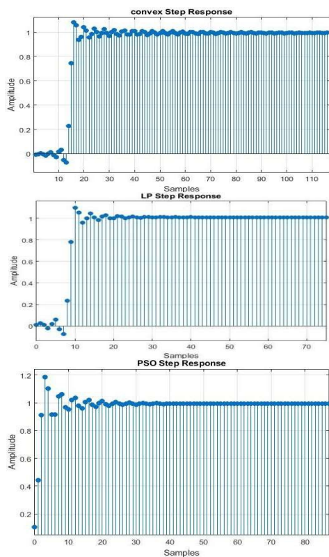
(شکل-۹): پاسخ پله فیلترهای PSO، Convex، و LP. Step response of designed filters by proposed, convex, and LP methods. (Figure-9)
