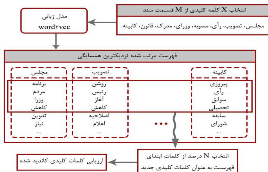
(Figure-6): How to identify new keywords using the suggested method
