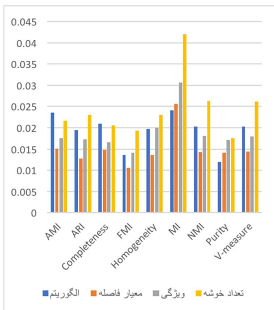
(Chart-2): Subtraction of HGPA from weighted HGPA by using w_1 and AD estimated
